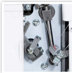
SELF-THREADING LOWER LOOPER
