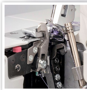
RETRACTABLE UPPER KNIFE
