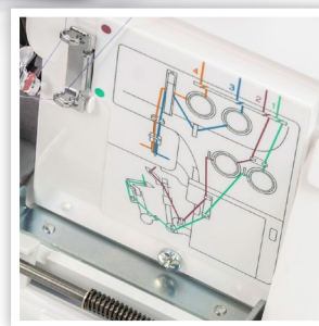
COLOUR CODED THREAD GUIDES
